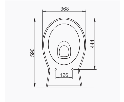
A021031 WC PAN WITHOUT BIDET FUNCTION
