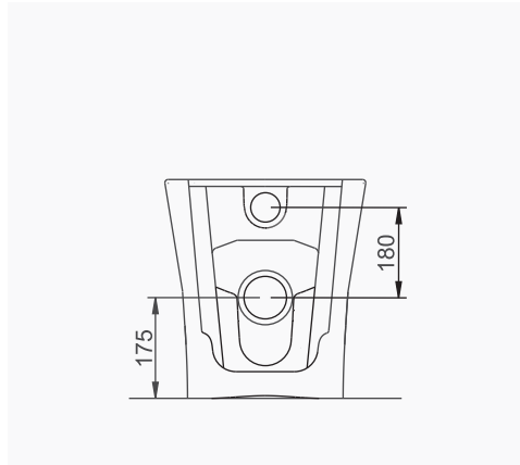
VOLCANO YERDEN TEK PARÇA KLOZET / VOLCANO SINGLE BTW WC PAN A021030 KLOZET / WC PAN A020011 YAVAŞ KAPANIR İNCE KAPAK / SLOW CLOSE SLIM SEAT & COVER
