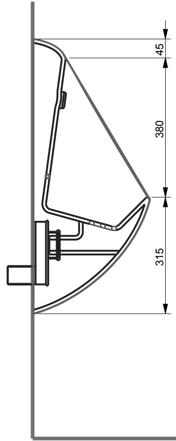
KESİT / SECTION
