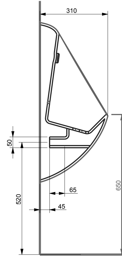
KESİT / SECTION
