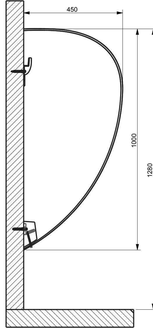
KESİT / SECTION
