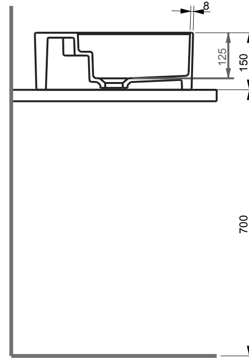
KESİT / SECTION
