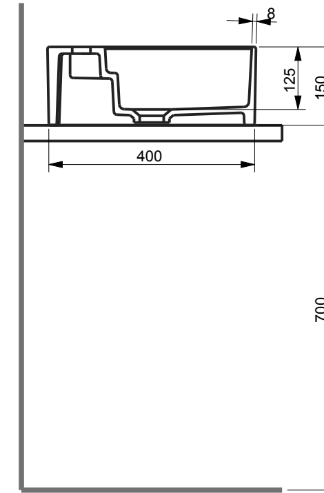
KESİT / SECTION
