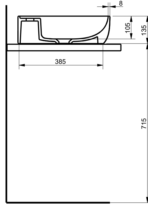
KESİT / SECTION
