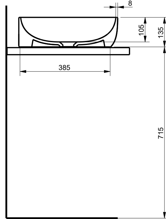
KESİT / SECTION
