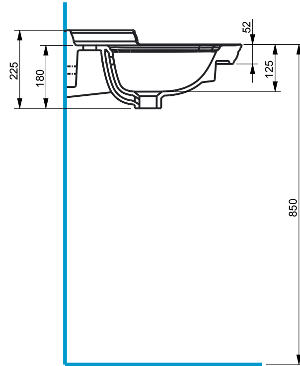
KESİT / SECTION
